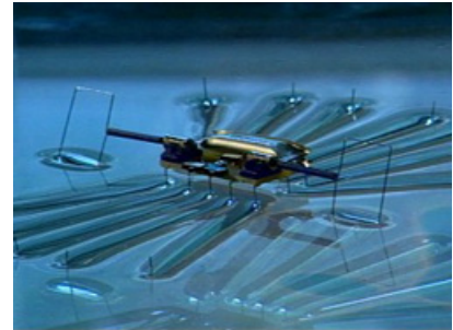
FIGURE 103 A water walking robot, total size about 20 mm (© AIP).
