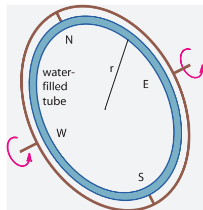
FIGURE 85 Demonstrating the rotation of the Earth with water.
