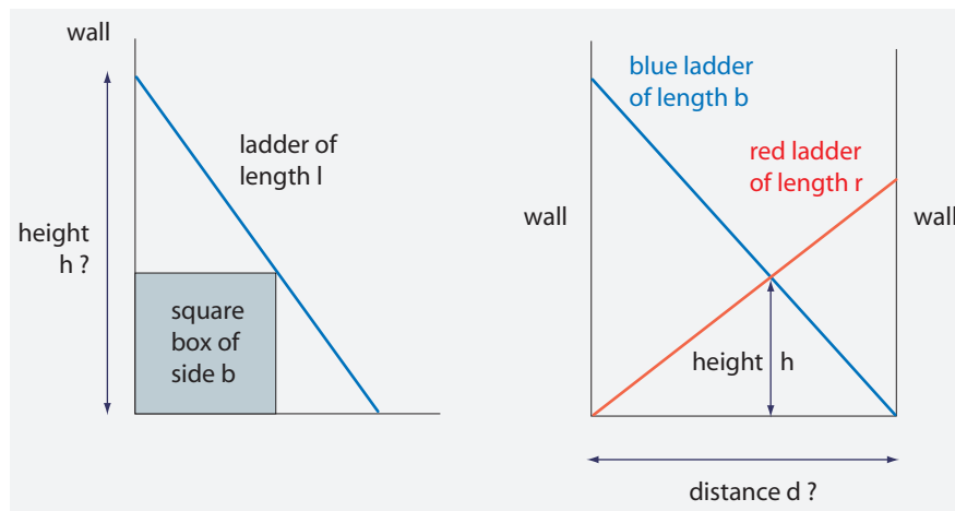
FIGURE 39 Two ladder puzzles: a moderately difficult (left) and a difficult one (right).
