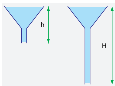
FIGURE 192 Which funnel is faster?
