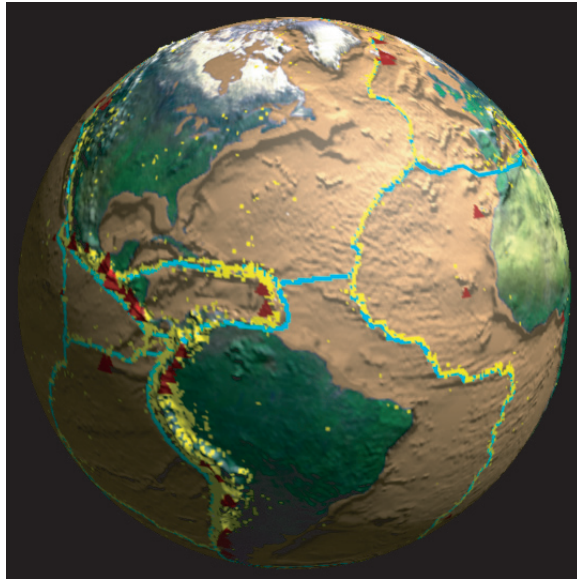
FIGURE 91 The continental plates are the objects of tectonic motion.
