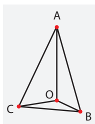
FIGURE 40 What is the area ABC, given the other three areas and three right angles at O?
