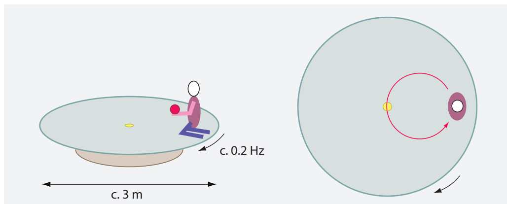
FIGURE 80 A typical carousel allows observing the Coriolis effect in its most striking appearance: if a person lets a ball roll with the proper speed and direction, the ball is deflected so strongly that it comes back to her.
