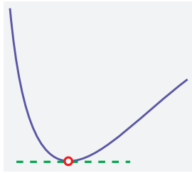
FIGURE 149 The minimum of a curve has vanishing slope.
