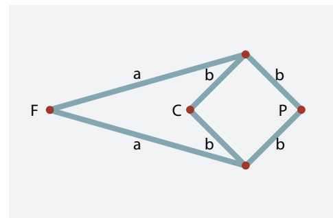
FIGURE 141 A famous mechanism, the Peaucellier-Lipkin linkage, that allows drawing a straight line with a compass: fix point F, put a pencil into joint P and move C with a compass along a circle.
