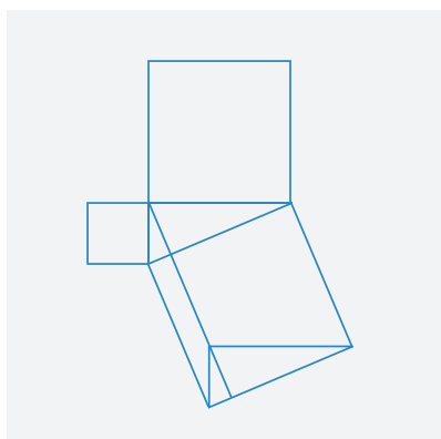
FIGURE 234 A simple drawing – one of the many possible one – that allows proving Pythagoras' theorem.
