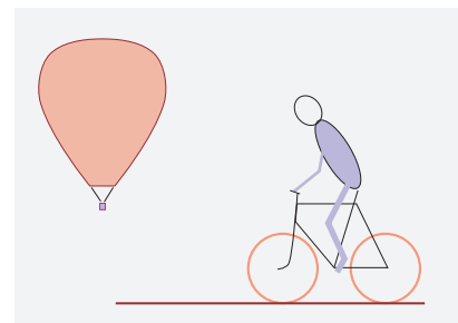
FIGURE 144 Why do hot-air balloons stay inflated? How can you measure the weight of a bicycle rider using only a ruler?
