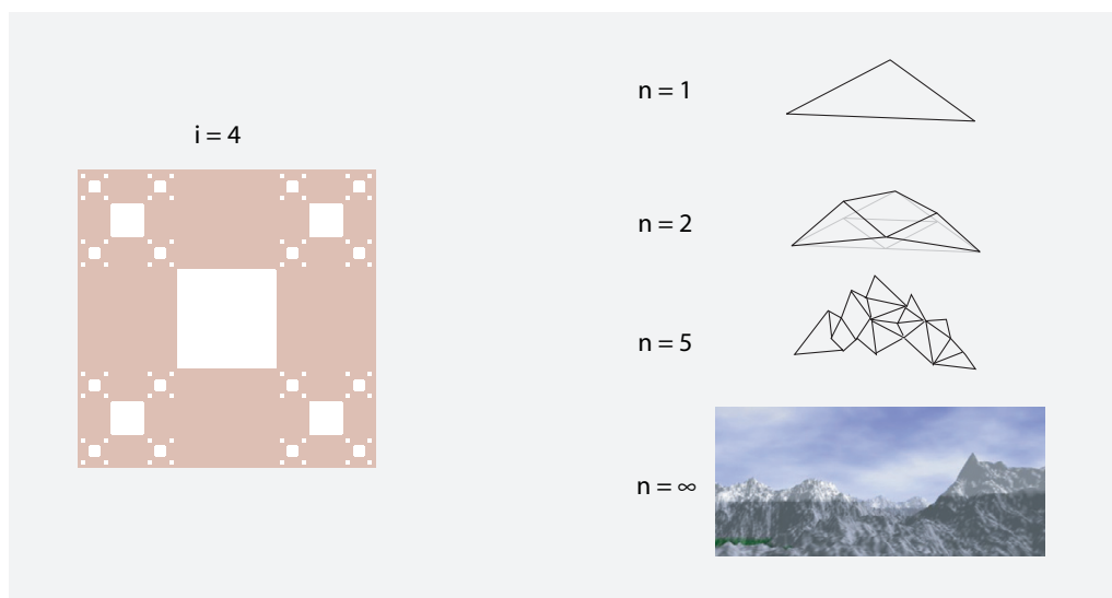
FIGURE 178 Floors (left) and mountains (right) could be fractals; for mountains this approximation is often used in computer graphics (image © Paul Martz).
