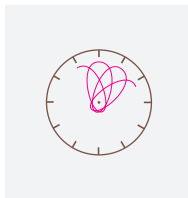
FIGURE 235 The trajectory of the middle point between the two ends of the hands of a clock.
