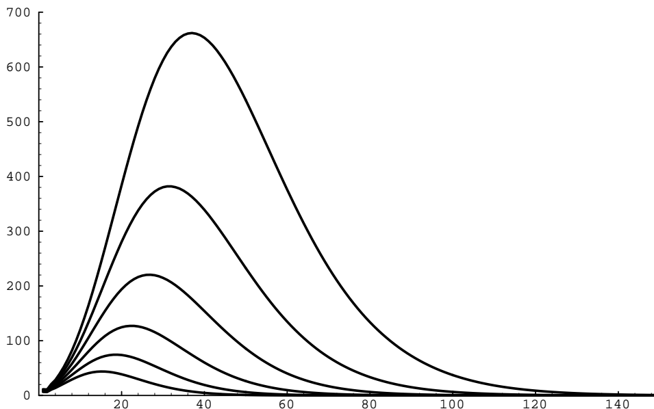
Figure 1: The distributions n_N(s, t_D) for N = 1K, 2K, 4K, \dots, 32K .
