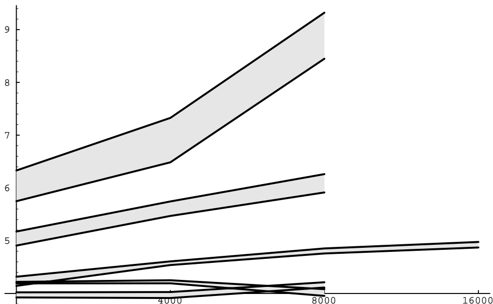
Figure 2: D_h(N, \kappa) shown as a function of N for (from top to bottom) \beta = -\frac{1}{2} \log \kappa = 0.14, 0.15 , ( N = 2K, 4K and 8K ), \beta^* \approx 0.1603 ( N = 2K, 4K, 8K and 16K ) and \beta = 0.17, 0.18 ( N = 2K, 4K and 8K ).
