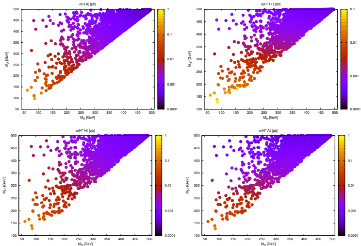
Figure : Production cross sections in pb at a 13 TeV LHC Tania Robens Extended scalar sectors, current and future Corfu2021, 1.9.21
