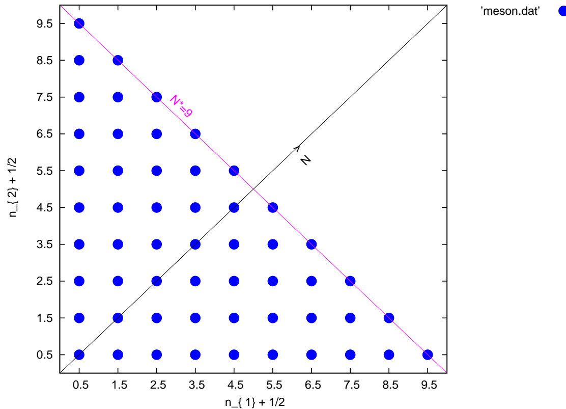
Fig. 2 : Illustration of partitions N = n_1 + n_2 simplifying the ones relevant for mesons
