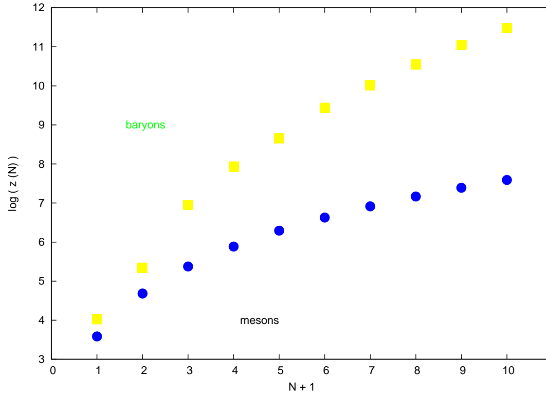
Fig. 3 : Density of states z(N) in logarithmic scale per unit mass-square \longleftrightarrow
