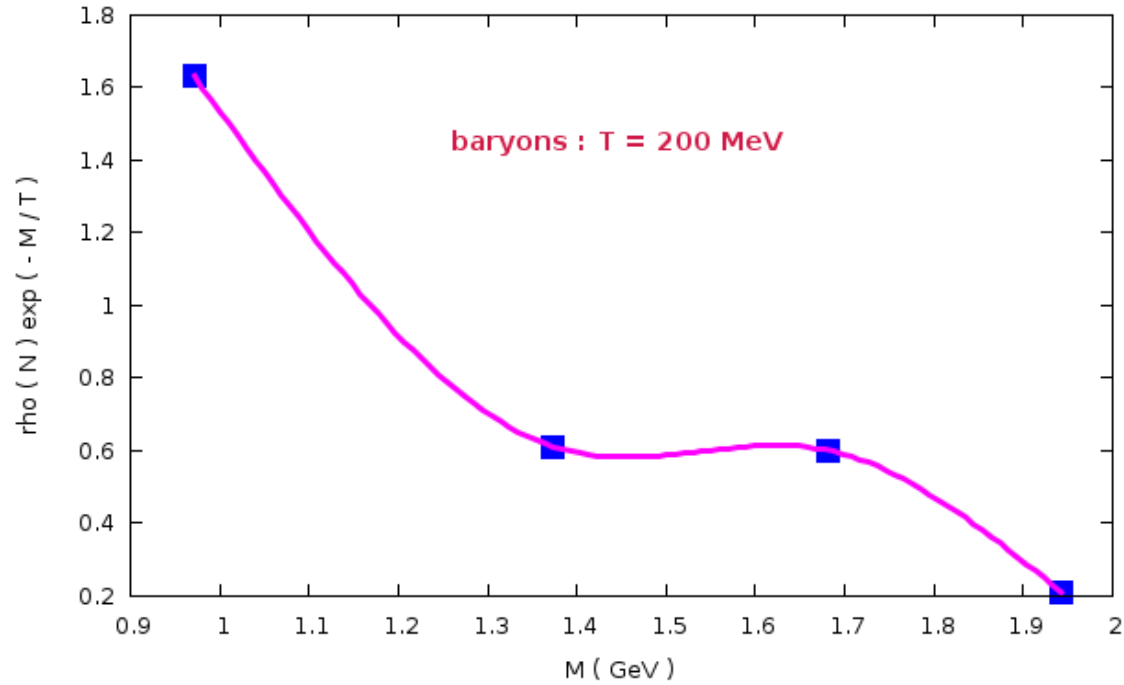
Fig. 4 : Density of states \rho(N) per unit mass-square for baryons weighted with the exponential factor \exp(-M/T) ; T : Temperature \longleftrightarrow
