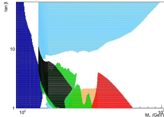
CMS Obs. gg H/A \rightarrow \tau\tau
